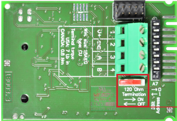
Bus termination resistor 120 Ω (ON-OFF slide switch)
