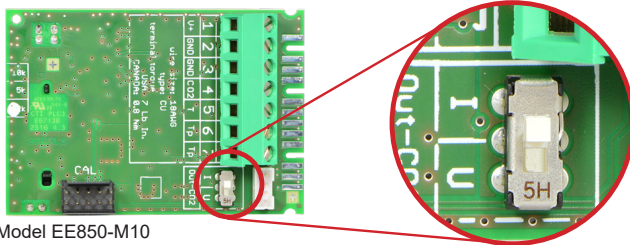
Model EE850-M10
