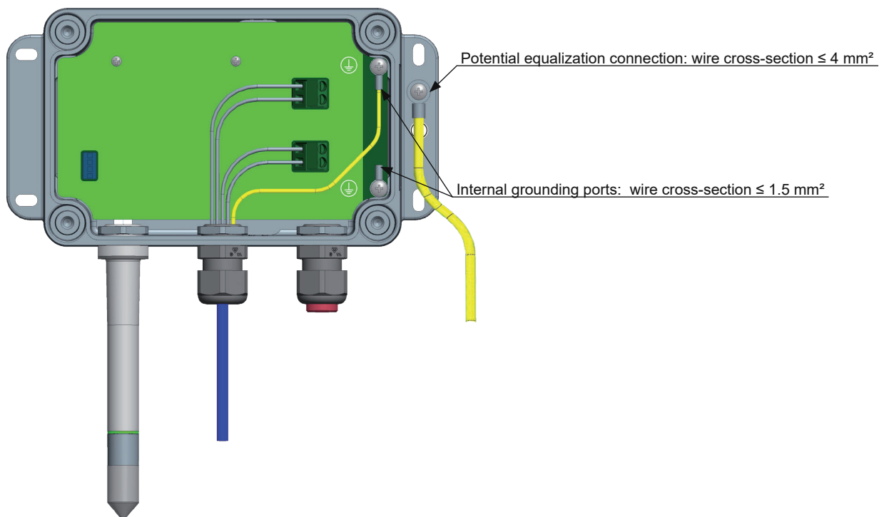
Fig. 4 Grounding and potential equalization
