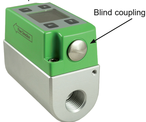
Fig. 15 Remove the blind cover
